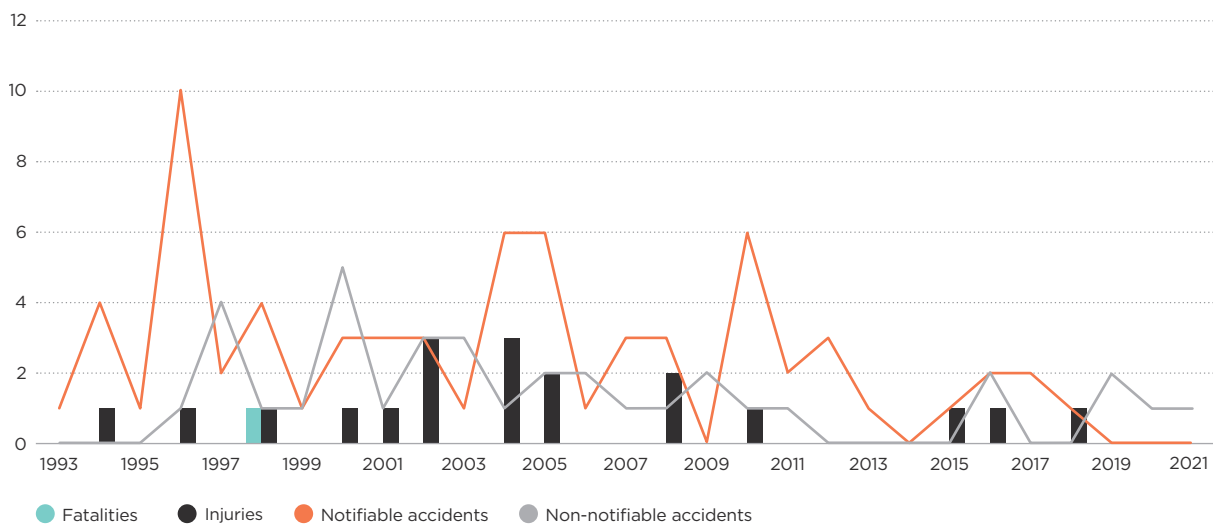
FIGURE 2I: Natural gas water heater and boiler accidents
