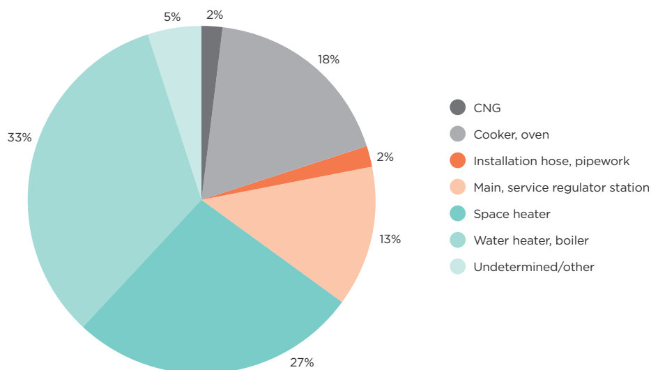
FIGURE 2E: Notifiable natural gas accidents by equipment
